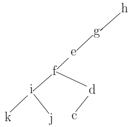
Tree defined by the parent pointers ( x and parent(x) ). Traverse this tree in Pre-order (root-left-right)
