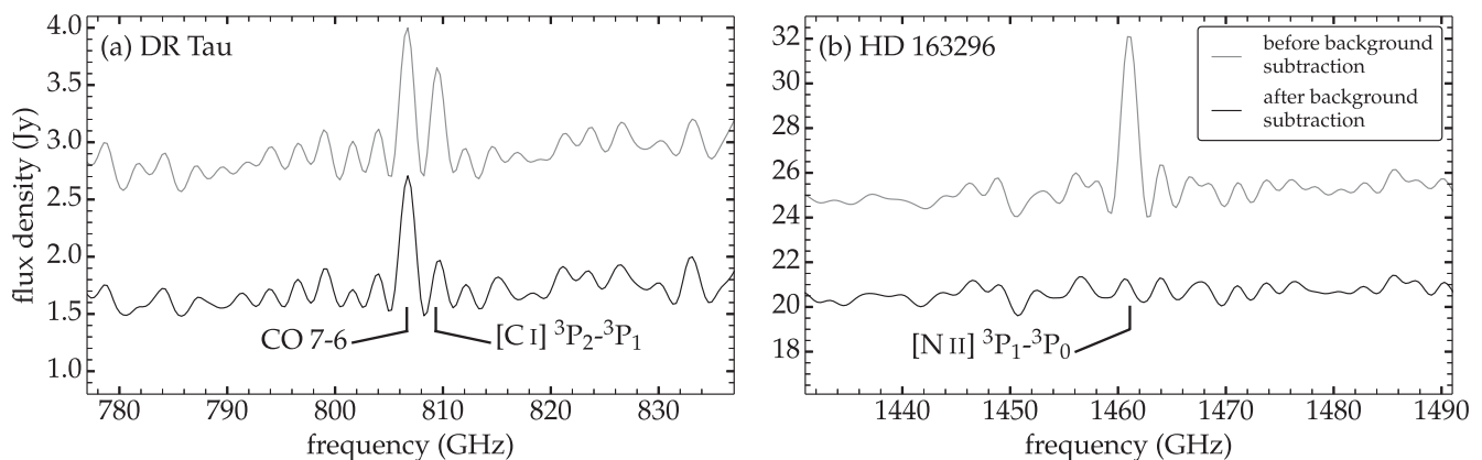
Figure 3. (a) Zoom of the 60 GHz section of the DR Tau spectrum centred around the CO 7–6 and [C I] ^3P_2 – ^3P_1 lines. The line of the neutral carbon atom coincides with the first sidelobe of the neighbouring CO line, but has significant flux of its own before background subtraction (grey), while its strength is reduced considerably after background subtraction is applied (black; same spectrum as in Fig. 2). (b) Zoom of the 60 GHz section of the HD 163296 spectrum centred around the [N II] line, again before and after background subtraction. This shows that the [N II] line towards HD 163296 originates from the extended background medium.
