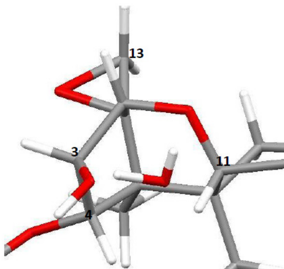
Figure 10. Proposed placement of water in the tetrahydropyranyl pocket of T-2 toxin. Cross-relaxation was observed between water and H-3, H-4 and H-11, indicating close proximity; chemical exchange between water and H-3 OH was also observed.
