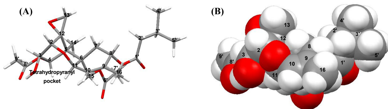
Figure 9. Solution and solid-state conformations. A model of the solution-state structure for T-2 toxin, showing the lowest energy conformation in the: (A) stick model; and (B) van der Waals representation. However, it is important to note here, that the side chains are flexible in the solution structure and are continuously moving, but the core ring structure is rigid; (C) Stick and (D) van der Waals representation for the Solid-state conformation 1, respectively; (E) Stick and (F) van der Waals representation for solid-state conformation 2. Note that the solid-state structure differ only in the torsion angles of the side chains; whereas, the solution state core structure differs substantially from the solid-state structures, particularly in the cyclohexene ring placement.
