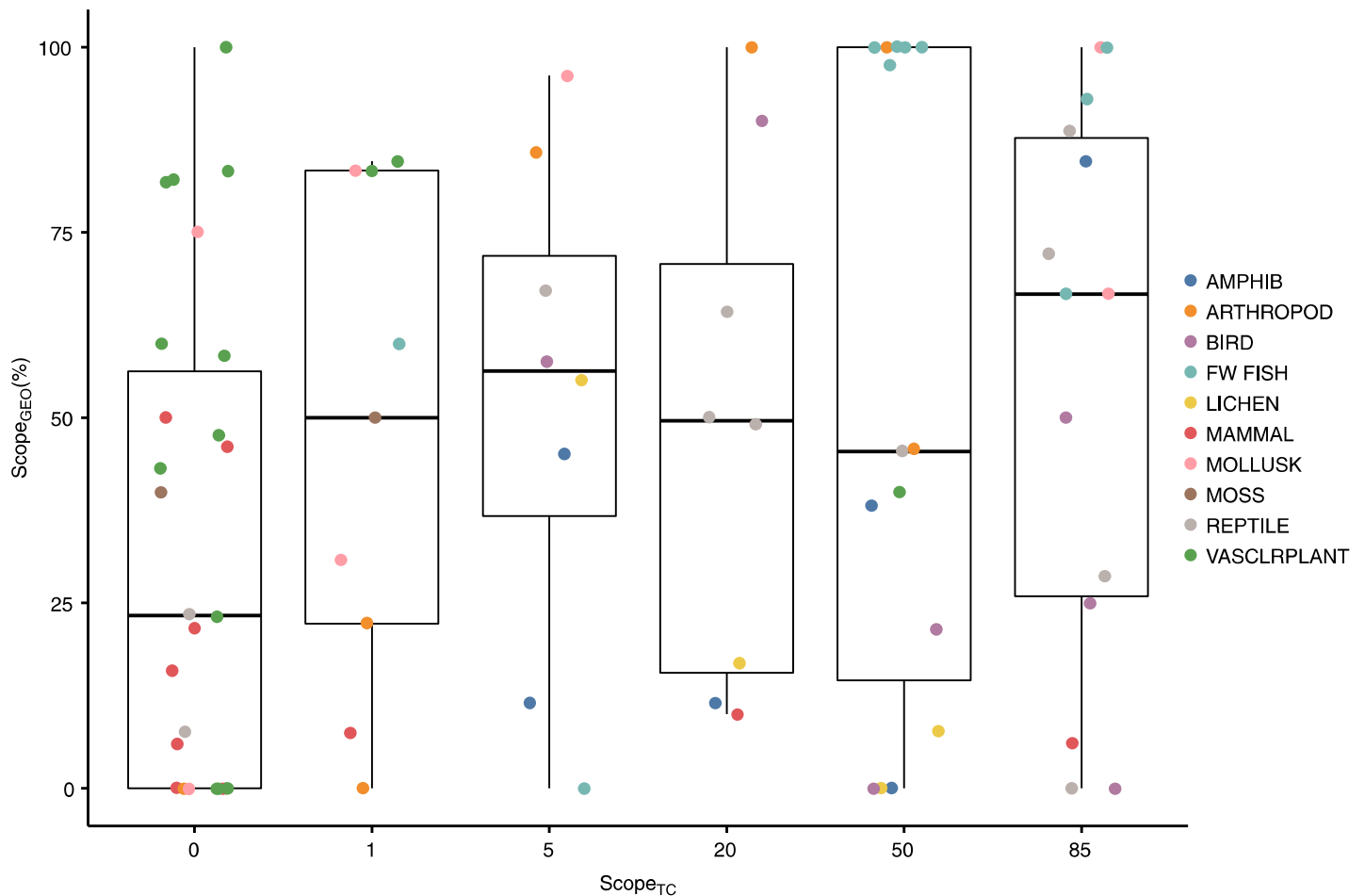
Fig. 4. The percentage of 100 km 2 cells occupied by a species that also contain one or more pollution sources ( scope_{GEO} ) plotted against the scope of pollution as assessed in Threats Calculators ( scope_{TC} ). N = 80 . AMPHIB, amphibians; FW FISH, freshwater fishes; VASCLRPLANT, vascular plants.
