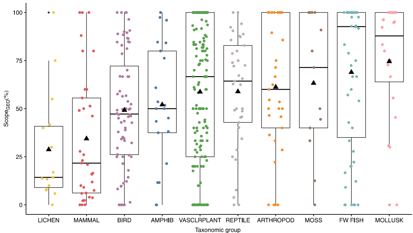
Fig. 2. The range in the percent overlap of pollution with species' occurrences ( scope_{GEO} )—considering all pollution categories together—by taxonomic group ( N = 488 ), in order of increasing mean scope. Triangles indicate the mean percent overlap for each taxonomic group. Thick horizontal lines indicate the median. AMPHIB, amphibians; VASCLRPLANT, vascular plants; and FW FISH, freshwater fishes.
