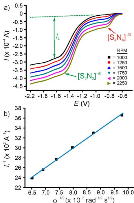
Figure 4. (a) RDE measurements on a 2.1 mM solution of S_2N_2 in CH_2Cl_2 with 0.4 M [nBu_4N][PF_6] at a 0.5 mm GC electrode, rotation rates = 1000 – 2250 RPM, v = 0.010 \text{ V s}^{-1} ; and (b) Koutecky-Levich 35 plot for the reduction of S_2N_2 ( R^2 = 0.998 ) after correction for S_4N_4 formation (see text).
