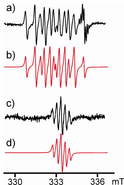
Figure 7. Experimental EPR spectra from single scans obtained during in situ reductive electrolysis of 1.5 mM S_2N_2 at -1.5 V (164 s single scan) at a platinum foil electrode in CH_2Cl_2 (0.4 M [^nBu_4N][PF_6] ) containing HBf_4 \cdot 2OEt_2 : (a) at -40 °C (black line) and (b) the simulation of this spectrum (red line); note that in the simulation the small contribution by [S_4N_4]^{+} (14% by area) has been omitted to more clearly show the high-field line component. (c) At -20 °C after about 10 minutes (black line). (d) Simulation (red line) of the spectrum in (c).
