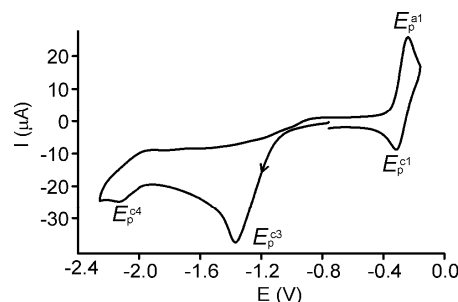
Figure 3. CV of a 2.0 mM soln of S_2N_2 in CH_2Cl_2 (0.4 M [nBu_4N][PF_6] ), v = 0.2 \text{ V s}^{-1} , T = 20^\circ\text{C} , with the potential sweep starting at -0.8 \text{ V} and extending further negative to include the second reduction process at -2.3 \text{ V} (labeled E_p^{c4} ).
