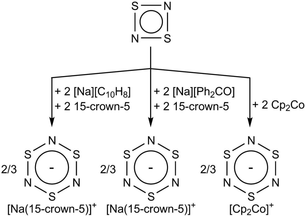
Formation of the [S_3N_3]^- anion from chemical reduction of S_2N_2 54x38mm (600 x 600 DPI)
