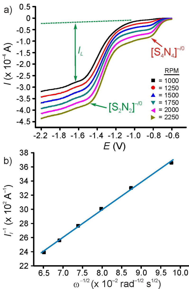
(a) RDE measurements on a 2.1 mM solution of S_2N_2 in CH_2Cl_2 with 0.4 M [nBu_4N][PF_6] at a 0.5 mm GC electrode, rotation rates = 1000 – 2250 RPM, v = 0.010 V s ^{-1} ; and (b) Koutecky-Levich 35 plot for the reduction of S_2N_2 ( R^2 = 0.998 ) after correction for S_4N_4 formation (see text).
