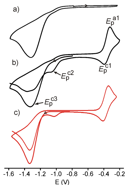
Figure 2. CVs (black lines) obtained on 2.0 mM solutions of \text{S}_2\text{N}_2 in \text{CH}_2\text{Cl}_2 containing 0.4 M [\text{nBu}_4\text{N}][\text{PF}_6] at a GC electrode at 20 °C, \nu = 0.2 \text{ V s}^{-1} with the potential starting at -0.8 V: (a) sweeping in the positive direction and (b) sweeping in the negative direction. (c) Calculated CV (red line) resulting from input of the kinetic parameters listed in the text for the specific case of \nu = 0.2 \text{ V s}^{-1} and k_{\text{B}} = 10^8 \text{ M}^{-1} \text{ s}^{-1} , sweeping the potential first in the negative direction starting at -0.8 V.
