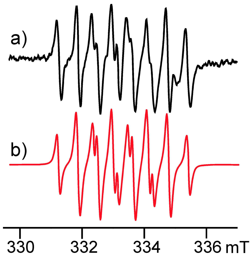
(a) Experimental EPR spectrum (black line) obtained during in situ reductive electrolysis of 1.5 mM S 2 N 2 at -1.5 V (164 s single scan) at a platinum foil electrode in CH 3 CN (0.1 M [nBu 4 N][PF 6 ]) at -20 °C after noise reduction, and (b) simulation (red line), with a(^{14}\text{N1}) = 1.12 mT, a(^{14}\text{N2}) = 0.65 mT, with a(^1\text{H}) = 0.60 mT, g value = 2.0136(1), mod. amp. = 0.2 mT. 82x83mm (600 x 600 DPI)
