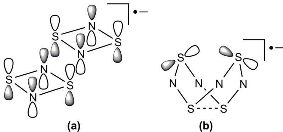
(a) Interaction between the LUMO of S 2 N 2 and the SOMO of [S 2 N 2 ] -• and (b) SOMO of the C 2v symmetric [S 4 N 4 ] -• radical anion. 34x16mm (600 x 600 DPI)
