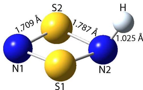
Figure 8. Optimized gas-phase UB3LYP/6-31G(d,p) structure of [\text{S}_2\text{N}_2\text{H}]^* ; \angle\text{S1-N1-S2} 94.7^\circ , \angle\text{N1-S1-N2} 87.8^\circ , \angle\text{S2-N2-S1} 89.4^\circ , \angle\text{S1-N2-H} 108.9^\circ , \angle\text{N1-N2-H} 120.4^\circ , \text{S1N1S2-S1N2S2} dihedral 6.9^\circ .
