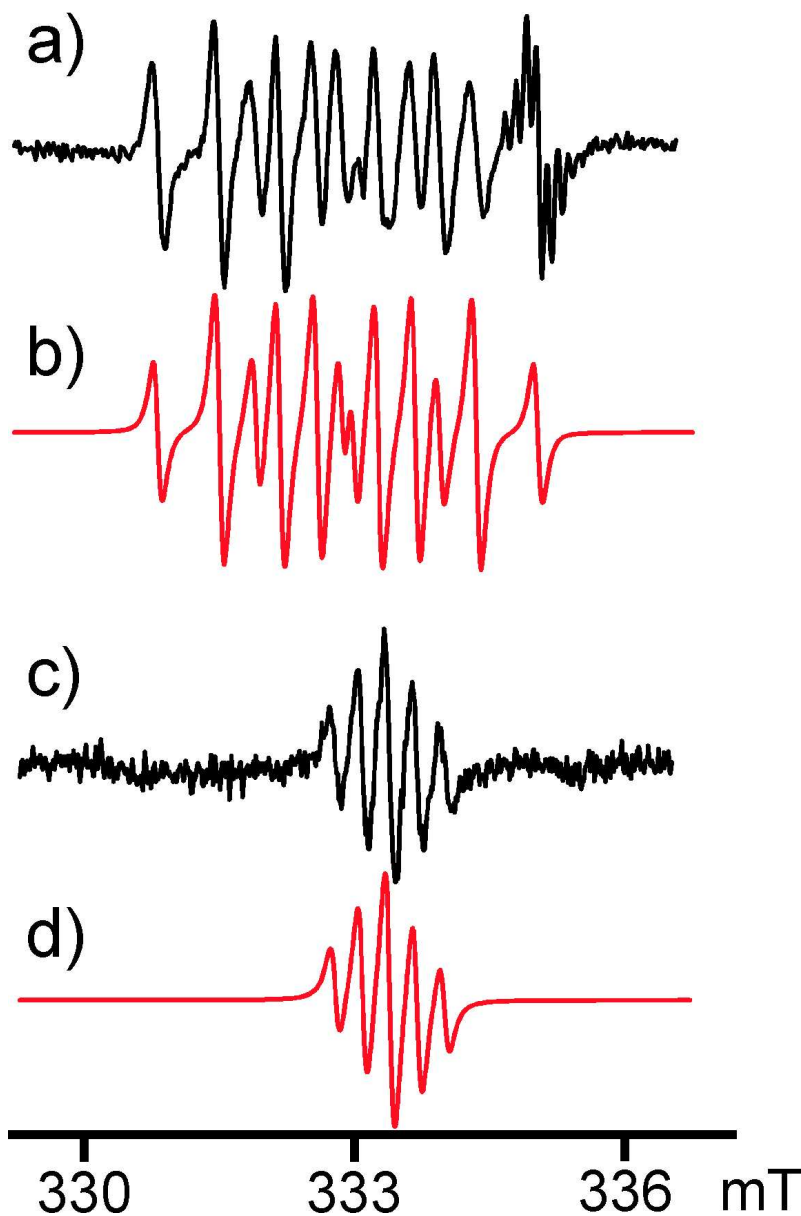
Experimental EPR spectra from single scans obtained during in situ reductive electrolysis of 1.5 mM S 2 N 2 at -1.5 V (164 s single scan) at a platinum foil electrode in CH 2 Cl 2 (0.4 M [nBu 4 N][PF 6 ]) containing HBF 4 •2OEt 2 : (a) at -40 °C (black line) and (b) the simulation of this spectrum (red line); note that in the simulation the small contribution by [S 4 N 4 ]-• (14% by area) has been omitted to more clearly show the high-field line component. (c) At -20 °C after about 10 minutes (black line). (d) Simulation (red line) of the spectrum in (c). 48x73mm (600 x 600 DPI)
