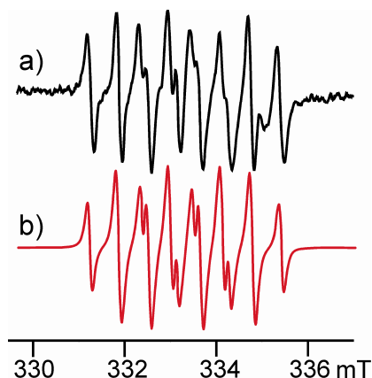
Figure 6. (a) Experimental EPR spectrum (black line) obtained during in situ reductive electrolysis of 1.5 mM \text{S}_2\text{N}_2 at -1.5 V (164 s single scan) at a platinum foil electrode in \text{CH}_3\text{CN} (0.1 M [\text{nBu}_4\text{N}][\text{PF}_6] ) at -20 °C after noise reduction, and (b) simulation (red line), with a(^{14}\text{N}_1) = 1.12 mT, a(^{14}\text{N}_2) = 0.65 mT, with a(^1\text{H}) = 0.60 mT, g value = 2.0136(1), mod. amp. = 0.2 mT.
