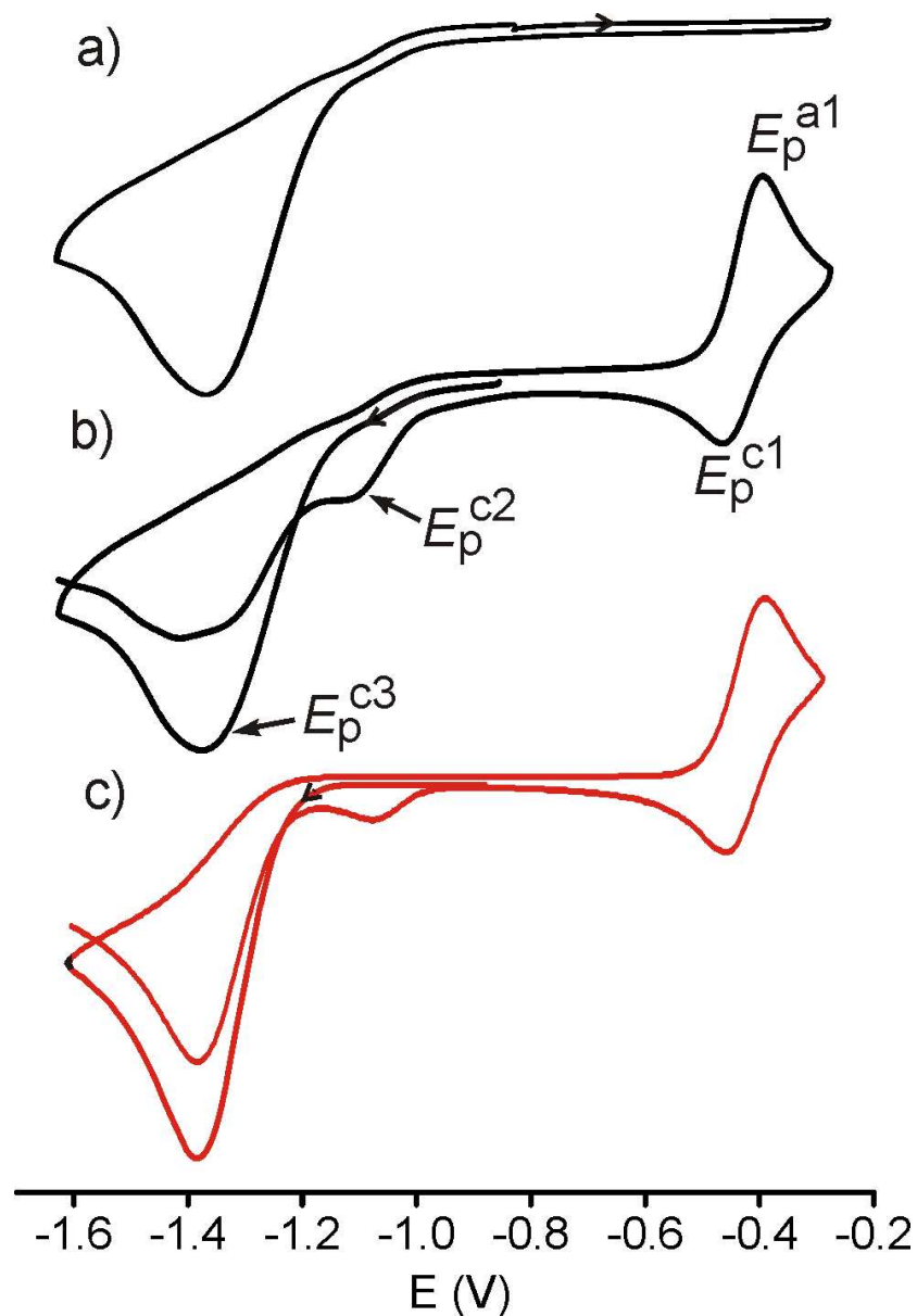
CVs (black lines) obtained on 2.0 mM solutions of S 2 N 2 in CH 2 Cl 2 containing 0.4 M [nBu 4 N][PF 6 ] at a GC electrode at 20 °C, \nu = 0.2 \text{ V s}^{-1} with the potential starting at -0.8 V: (a) sweeping in the positive direction and (b) sweeping in the negative direction. (c) Calculated CV (red line) resulting from input of the kinetic parameters listed in the text for the specific case of \nu = 0.2 \text{ V s}^{-1} and kf_3 = 108 \text{ M}^{-1} \text{ s}^{-1} , sweeping the potential first in the negative direction starting at -0.8 V. 82x120mm (300 x 300 DPI)
