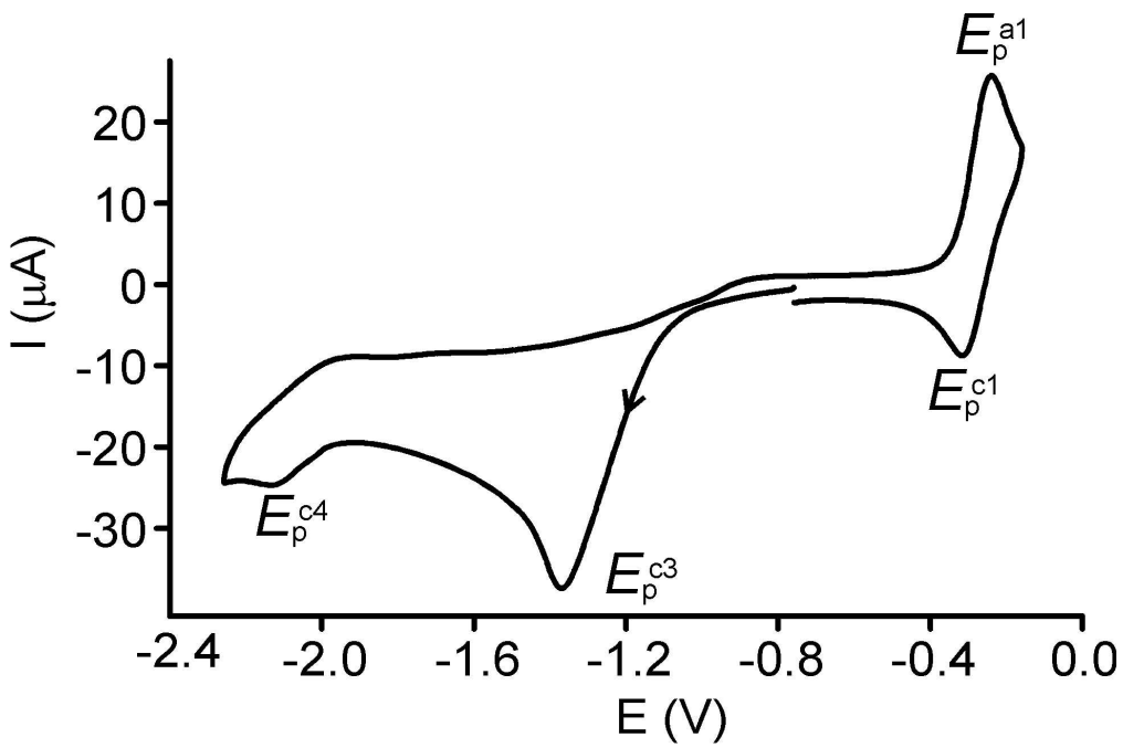
CV of a 2.0 mM soln of S 2 N 2 in CH 2 Cl 2 (0.4 M [nBu 4 N][PF 6 ]), \nu = 0.2 \text{ V s}^{-1} , T = 20 \text{ }^{\circ}\text{C} , with the potential sweep starting at -0.8 \text{ V} and extending further negative to include the second reduction process at -2.3 \text{ V} (labeled E pc4 ). 82x54mm (600 x 600 DPI)
