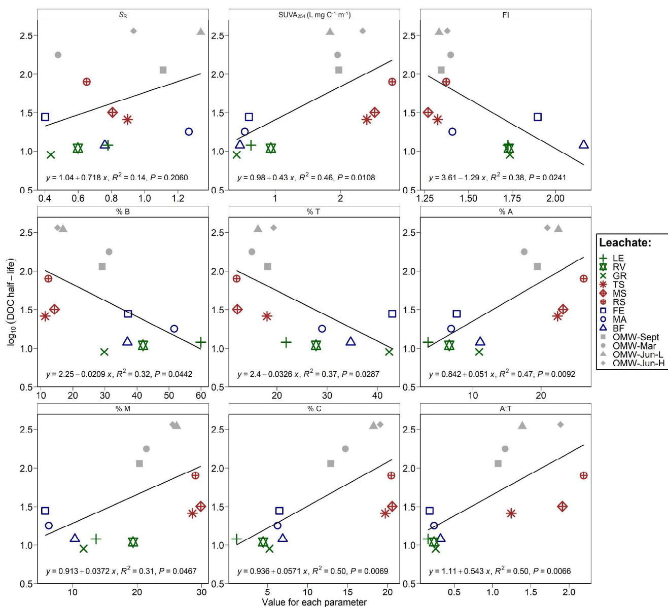
Figure 5. Relationship between \log_{10}(\text{half-life}) to bulk optical parameters including individual absorbance metrics ( S_R , SUVA 254 , and fluorescence index) and the percent individual peak (B, T, A, M, C) contribution to F_{\text{max}} .
