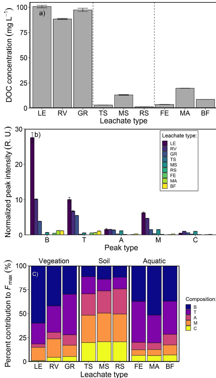
Figure 3. Initial (a) dissolved organic carbon concentration, and Raman normalized fluorescent peak (b) intensities and (c) percent contribution to F_{\max} for all leachates, including 3 vegetation types (LE, RV, and GR for leaf, riparian vegetation, and grass leachates, respectively), 3 surface soil types (RS, MS, and TS for leachates from soils at riparian, mid-valley, and top of valley locations, respectively), and 3 aquatic dissolved organic matter (DOM) sources (FE, MA, and BF, for fish excretion DOM, and macrophyte and biofilm leachates, respectively). Each bar represents the average of triplicate measurements, where error bars are \pm 1 standard deviation.
