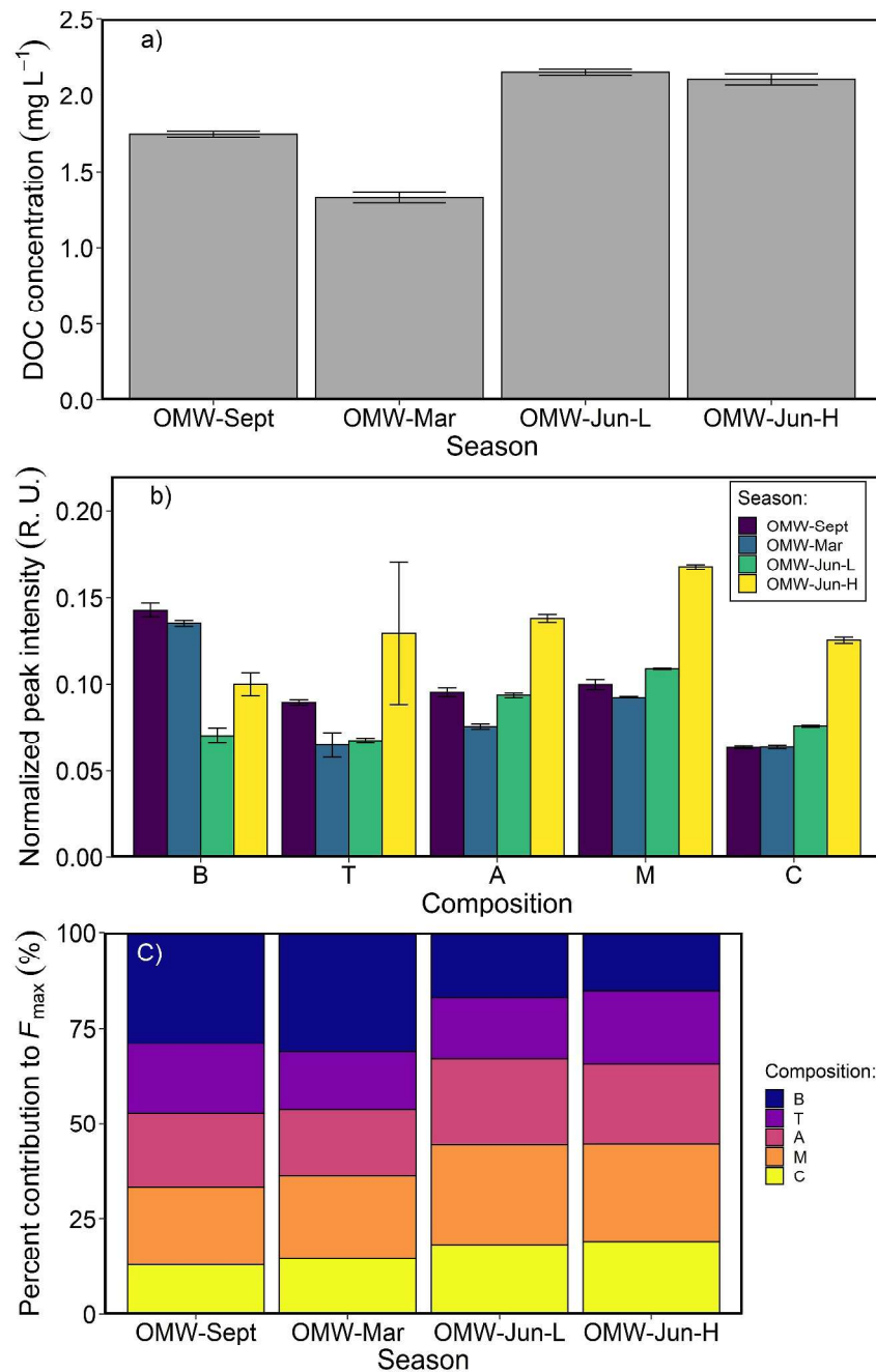
Figure 2. Initial (a) dissolved organic carbon concentration, and Raman normalized fluorescent peak (b) intensities and (c) percent contribution to F_{\max} , for the Oldman River across seasons: September (OMW-Sept), March (OMW-Mar), June low flow (OMW-Jun-L), and June Spring flood (OMW-Jun-H). Each bar represents the average of triplicate measurements, where error bars are \pm 1 standard deviation.
