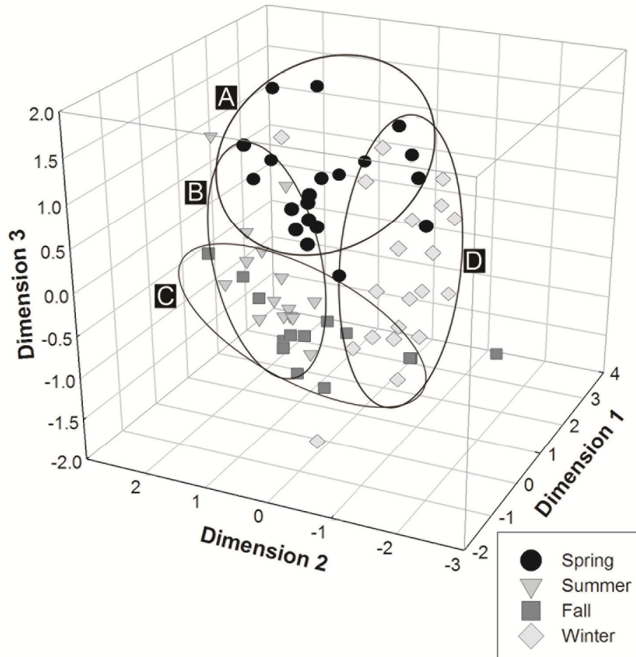
Figure 4.4. Non-metric multidimensional scaling plots of T-RFLP community profiles from river water (stress = 14) with ellipses A-D encompassing 90 % of respective markers by season; markers that appear close together are more similar than distant markers.
