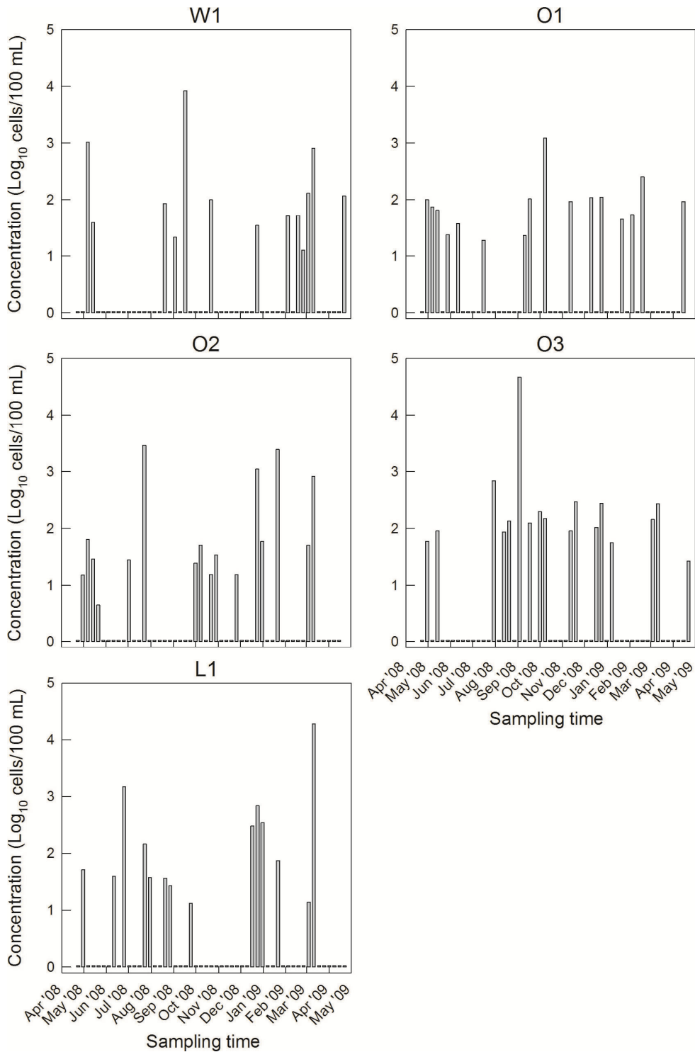
Figure 3.3. Estimation of C. jejuni cell densities (Log 10 cells per 100 mL) in river water by qPCR. Sites are: Oldman River downstream of Fort McLeod (O1); Oldman River downstream of Lethbridge (O2); Oldman River under the Highway 845 bridge (O3); Little Bow River near the confluence with the Oldman River (L1); and Willow Creek north of Fort McLeod (W1). See Figure 3.1 for additional information on the sites.
