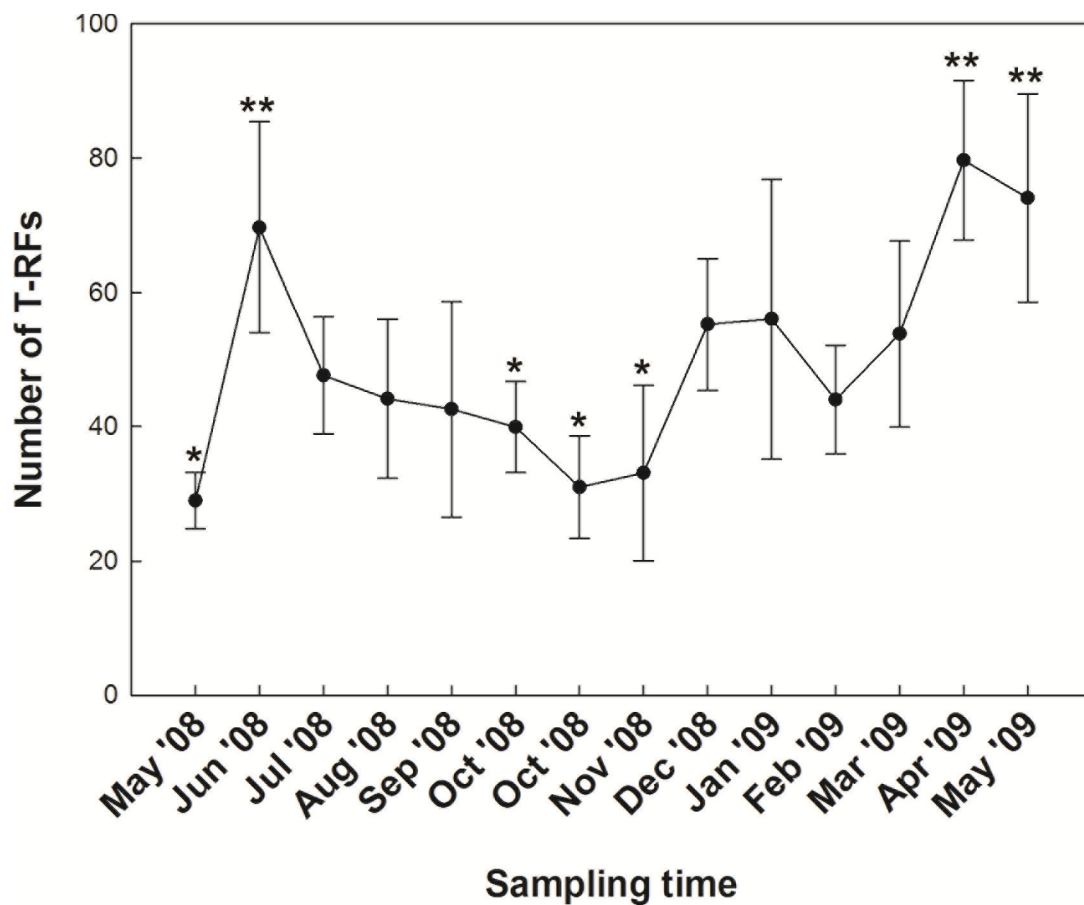
Figure 4.2. Number of terminal restriction fragments over a one year sampling period (May of 2008 to May of 2009). Vertical bars associated with means represent the standard deviation across the five sample sites. Means denoted with a single asterisk differ ( P \leq 0.05 ) from means indicated by a double asterisk.
