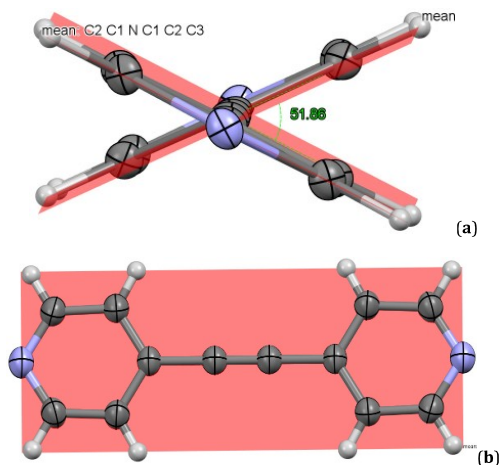
Figure 3. Dihedral angles of the two pyridyl planes in 1 (a) and 1a (b).
