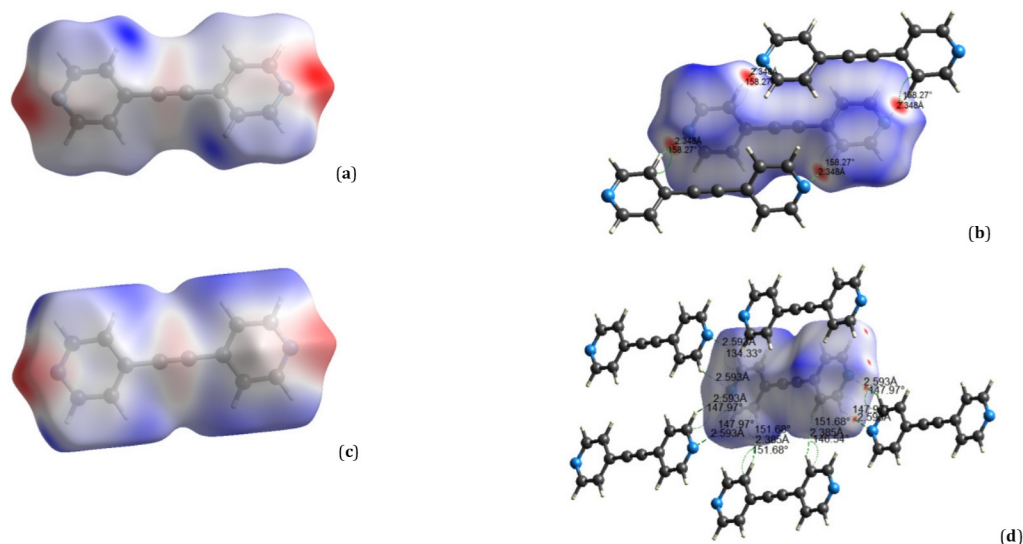
Figure 6. The Hirshfeld surface of 1 and 1a mapped on (a) an ESP surface (a, c) showing the negative and positive ESP regions indicative of proton acceptor and donor potentials, respectively (b) d_{\text{norm}} (b, d) showing four red hotspots identifying C_{\text{pyr-meta}}\text{H}\cdots\text{N}_{\text{pyr}} contacts in 1 and eight symmetrically distributed red hotspots attributed to C_{\text{pyr-ortho}}\text{H}\cdots\text{N}_{\text{pyr}} HBIs that are shorter than the summation of the van der Waals radii of nearest neighbor atoms.
