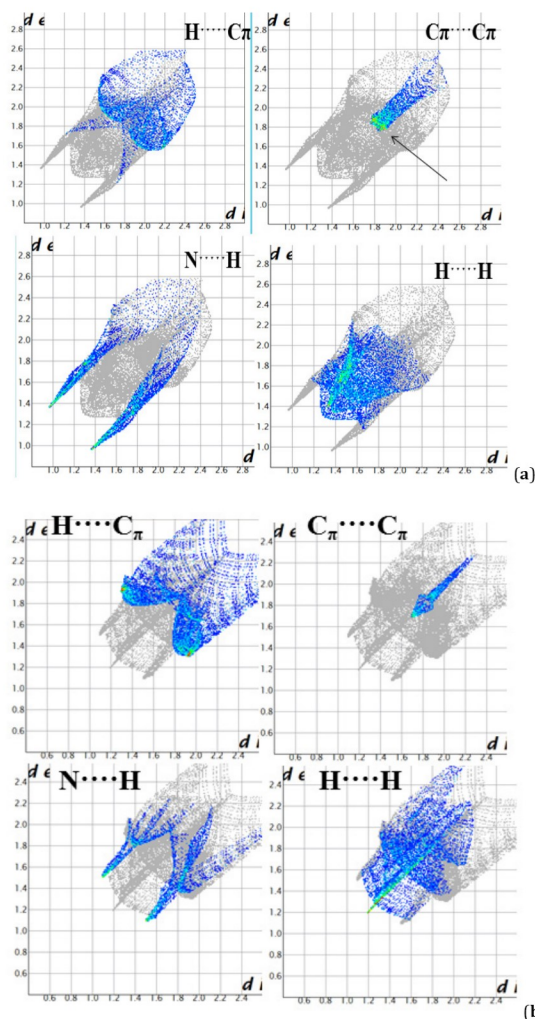
Figure 7. (i) H\cdots C\pi : wings on FPs, (ii) C\pi\cdots C\pi : hot points distributed in d_i - d_e region of FPs, (iii) N\cdots H : wings located between spikes and external wings and (iv) H\cdots H : mandibular splitting of the non-bonding contacts located between spikes or antennae for 1 (a) and 1a (b).
