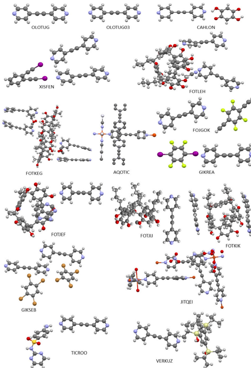
Figure 4. Co-crystals and metal complexes containing compound 1 (Solvates have been omitted for clarity).
