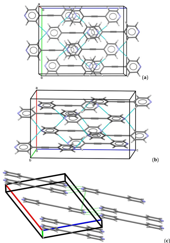
Figure 5. Packing motifs of structures 1 (a, b) and 1a (c) showing the 2D array of repeated dimeric pairs antiparallel-displaced monomeric units (a) connected by edge-to-edge \text{C}_{\text{pyr}}\text{-H}\cdots\text{N}_{\text{pyr}} supramolecular synthons (b) and the close to planar layers formed from corrugated ribbons of intermolecular interactions (c) revealing the close proximity of monomeric units necessary for the interaction of non-attractive atoms such as H and \text{C}_{\pi} of the pyridyl periphery.
