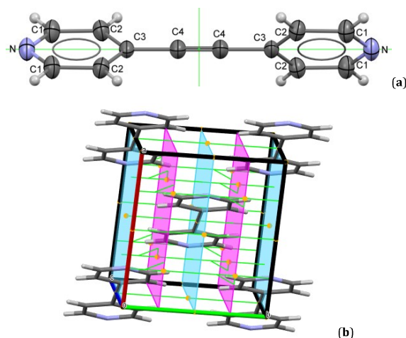
Figure 2. Alignments of the symmetry elements in 1 (a) and 1a (b) with symmetry components: Mirror planes (light blue), Glide planes (purple), 2-fold and proper rotation axes (green), Inversion centers (yellow).
