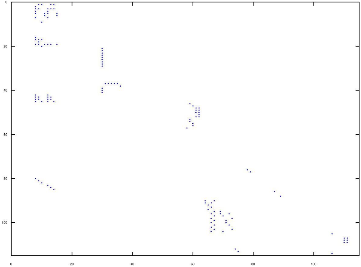
Figure 4.11: ADOL-C, sparse matrix
