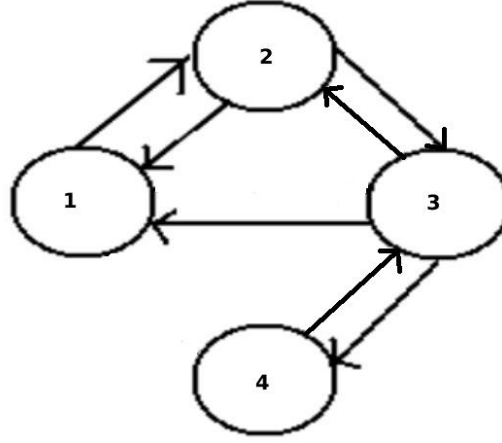
Figure 3.1: Directed network
