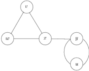
Figure 2.8: Undirected graph
