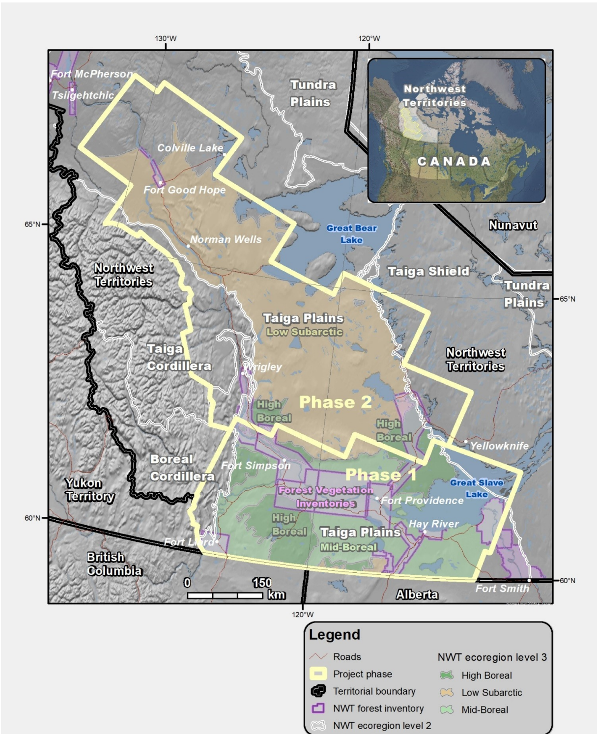
Figure 1. Overview of the Multisource Vegetation Inventory (MVI) project area. The ~151,700 km 2 Phase 1 has 2007 as the reference year, covers mostly the Taiga Plains Mid-Boreal (light green) and HighBoreal (dark green) ecoregions, and overlaps with ~36,600 km 2 of Government of the Northwest Territories (GNWT) Forest Vegetation Inventories (FVIs, purple polygons). The 244,000 km 2 Phase 2 has 2010 as the reference year, covers mostly the Taiga Plains Low Subarctic Ecoregion (brown), and overlaps with ~9500 km 2 of GNWT FVIs. Main populated places are shown as white dots.
