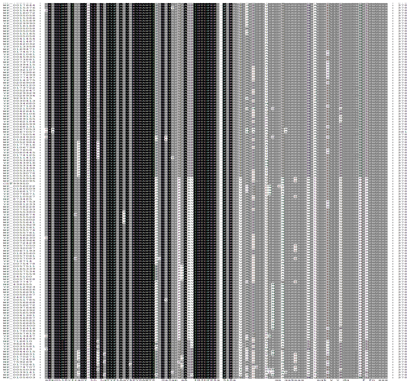
Figure A.2 Alignment of 291 bacterial YchF primary sequences. Black indicates 100% identity, dark grey 80 to 100-conservation, light grey 60 to 80% and white shading is indicative of less than 60% identity.
