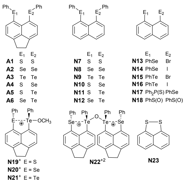
Chart 2. Structures and substituents for the investigated compounds.
