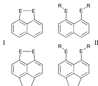
Chart 1. Two major types of chalcogen-substituted naphthalenes (top) and acenaphthenes (bottom).
