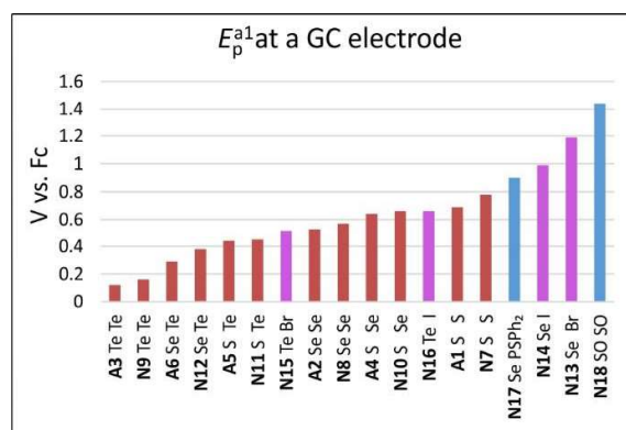
Fig. 4. Bar graphs showing the large increase in E_p^{a1} values found for A1 – N18 as a function of E/X groups measured at a GC electrode interface. (For data measured at a Pt electrode, see ESI).
