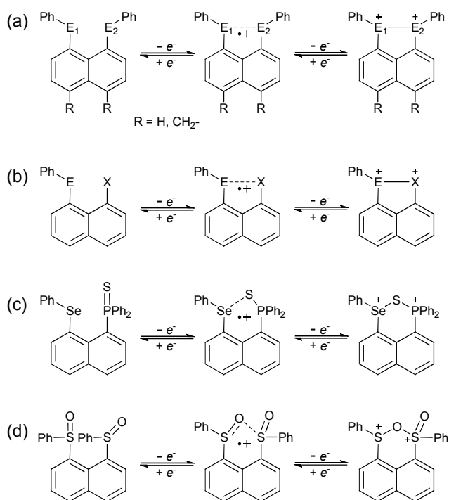
Scheme 3. ETMs for oxidation of peri -disubstituted diaryl dichalchogenides A1 – N12 to form new bonds.
