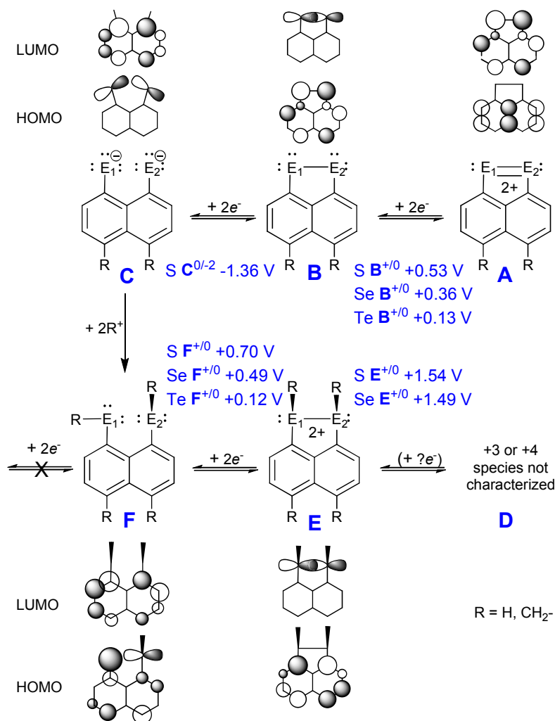
Fig. 12. Comparative RMOs of the Type I and Type II dichalcogen naphthalene/acenaphthenes correlated to the redox transformations, expressed as standard reductions for the putative 2e^- transformations.
