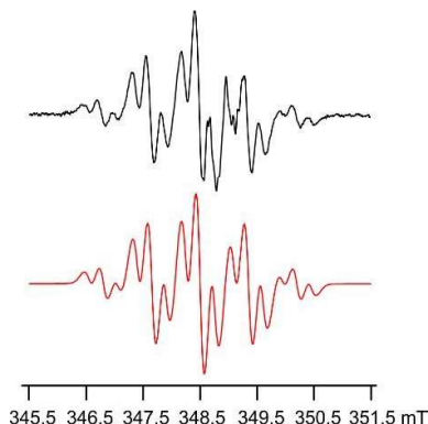
Fig. 3. Top: EPR spectrum of A1 •+ obtained in CH 2 Cl 2 by oxidation with NOBF 4 (from 100 accumulated scans through the indicated field range). Bottom: Simulation undertaken with WinSim2000 (in red). 67
