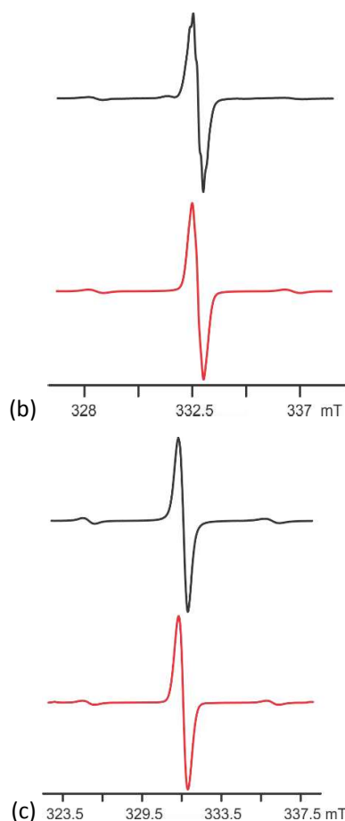
Fig. 2. SEPR spectra (in black) obtained in \text{CH}_2\text{Cl}_2/0.1 \text{ M } [{}^n\text{Bu}_4\text{N}][\text{PF}_6] with an in situ EPR electrochemical cell. Spectra are from single scans through the indicated field ranges, while electrolysis is undertaken on (a) N7 , (b) N10 and (c) N8 . Simulations with line-fitting were undertaken with WinSim2000 (in red). 67
