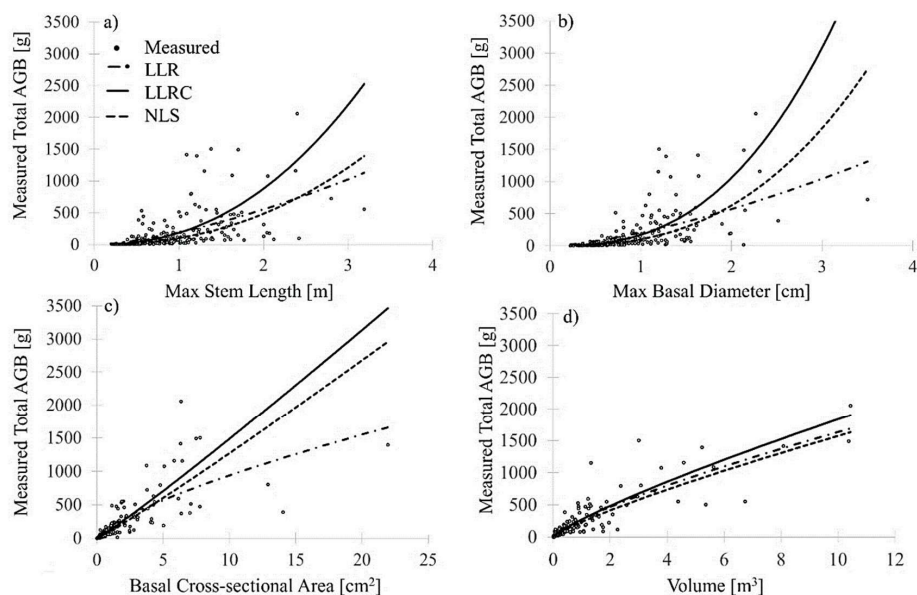
Figure 3. LLRC, LLR, and NLS model fits for each 1D (a,b), 2D (c), and 3D (d) predictor variable utilized to model total AGB for multispecies shrubs.
