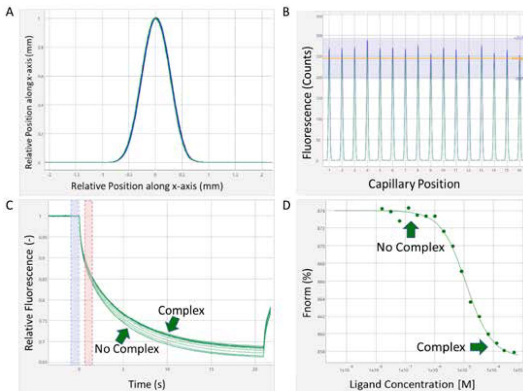
Figure 2. Microscale thermophoresis outputs. Plots visualizing several MST outputs from different experiments.
