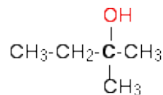
2-methylbutan-2-ol
