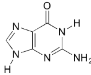
guanine (G)
