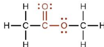
methyl ethanoate (methyl acetate)
