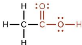
ethanoic acid (acetic acid)
