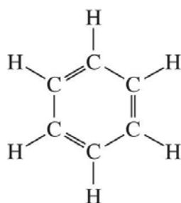
Kekulé structure for benzene
