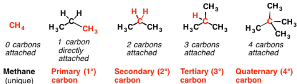
Figure 1. https://www.masterorganicchemistry.com/2010/06/16/1°-2°-3°-4°/
