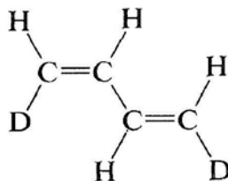
(1Z,3E)-1,3-butadiene-1,4- d_2
