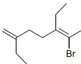
6-bromo-2,5-diethyl-1,5-hepta a diene, or 6-bromo-2,5-diethyl-hepta a -1,5-diene
