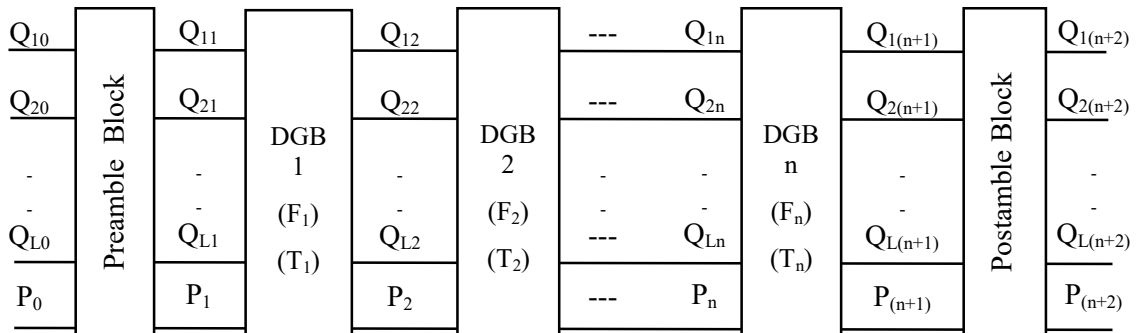
Figure 4.21: Block diagram of an online testable reversible circuit.
