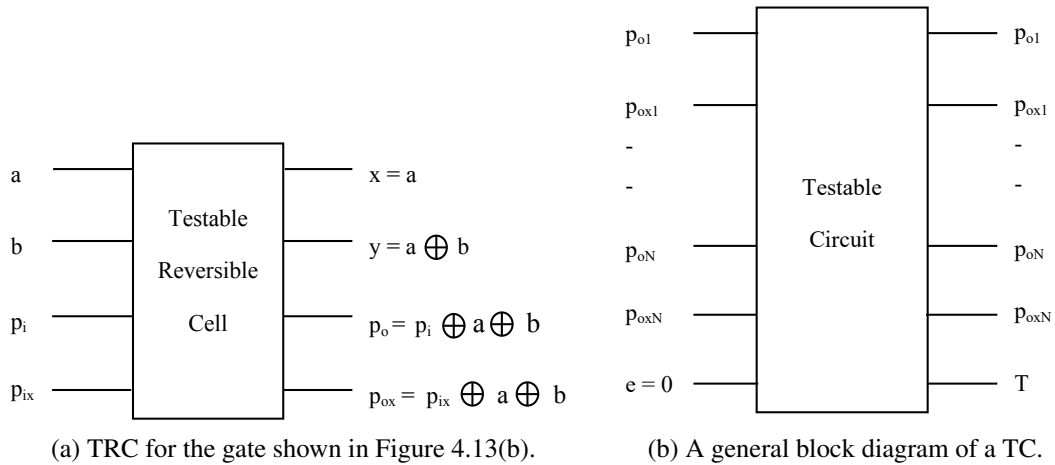
Figure 4.14: TRC and TC for online testability.
