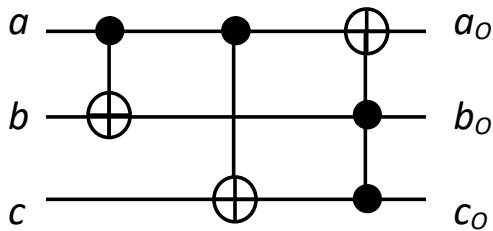
Figure 5.7: A reversible majority voter as proposed in [6].
