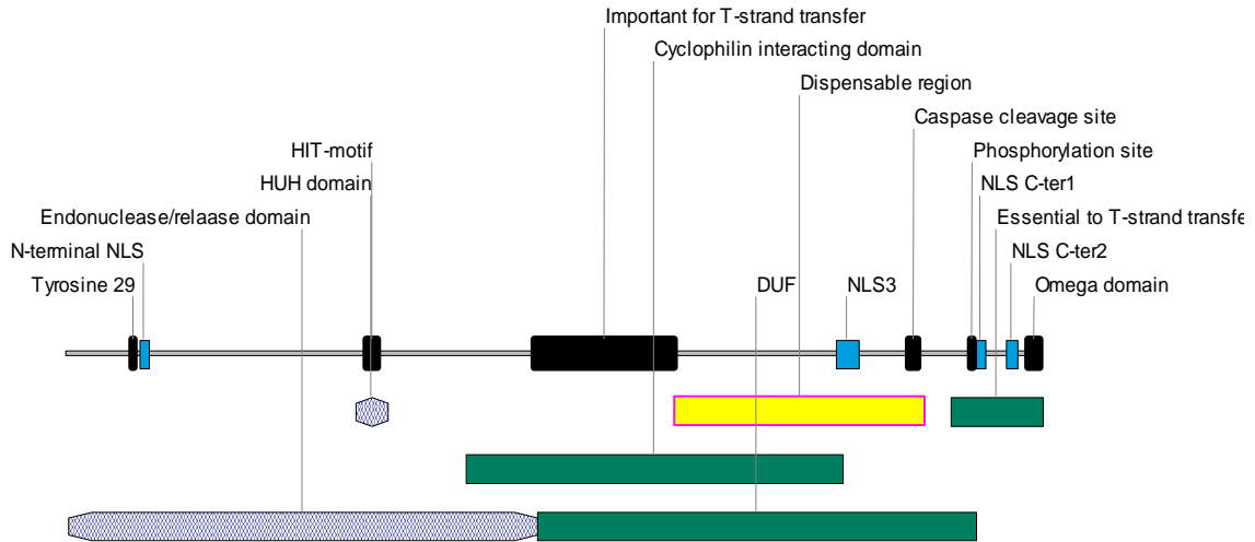
Figure 1.4. Schematic representation of VirD2 with domains and motifs. NLS C-ter1 and NLS C-ter2: the C-terminal bipartite NLS. NLS3 (see Chapter 3).
