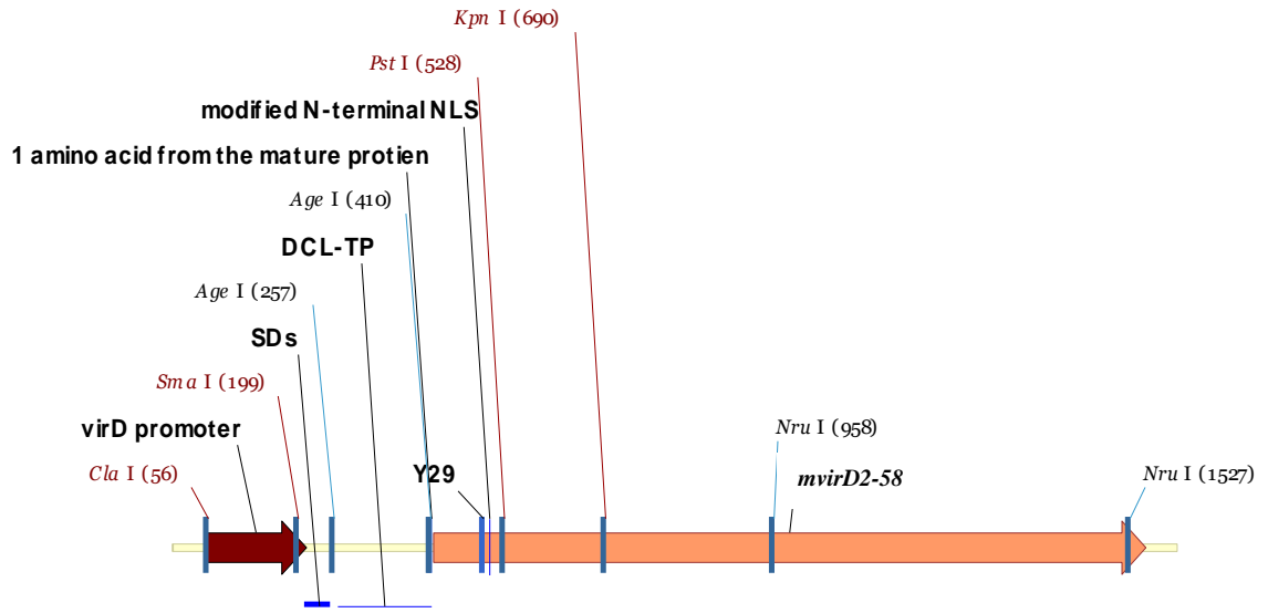
Figure 2.4.1b. Schematic representation of the DCL-TP-mvirD2-58 gene in pVD58-DCI-TP. SD: the Shine-Dalgarno sequence; some restriction sites are shown.
