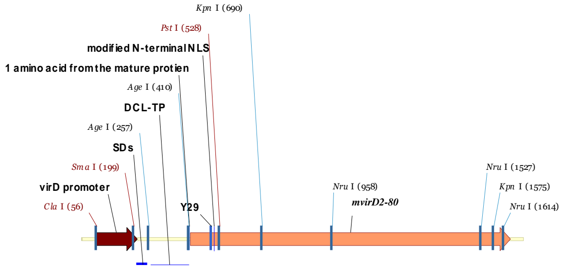
Figure 2.4.1d. Schematic representation of the DCL-TP-mvirD2-80 gene in pVD80-DCI-TP. SD: the Shine-Dalgarno sequence; some restriction sites are shown.
