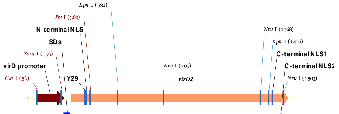
Figure 2.4.1a. Schematic representation of the virD2 gene in pVD43. SD: the Shine-Dalgarno sequence; C-terminal NLS1 and 2: C-terminal bipartite NLS; some restriction sites are shown.
