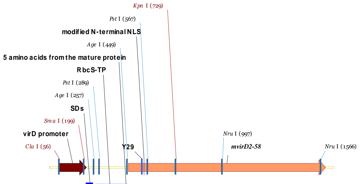
Figure 2.4.1c. Schematic representation of the RbcS-TP-mvirD2-58 gene in pVD58-RbcS-TP. SD: the Shine-Dalgarno sequence; some restriction sites are shown.
