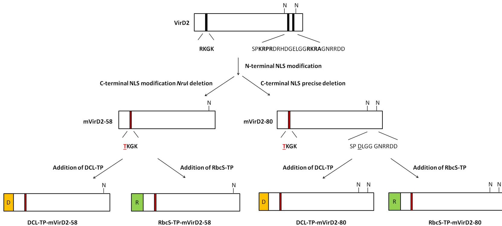
Figure 2.4.2a. Construction scheme of TP-mVirD2.
