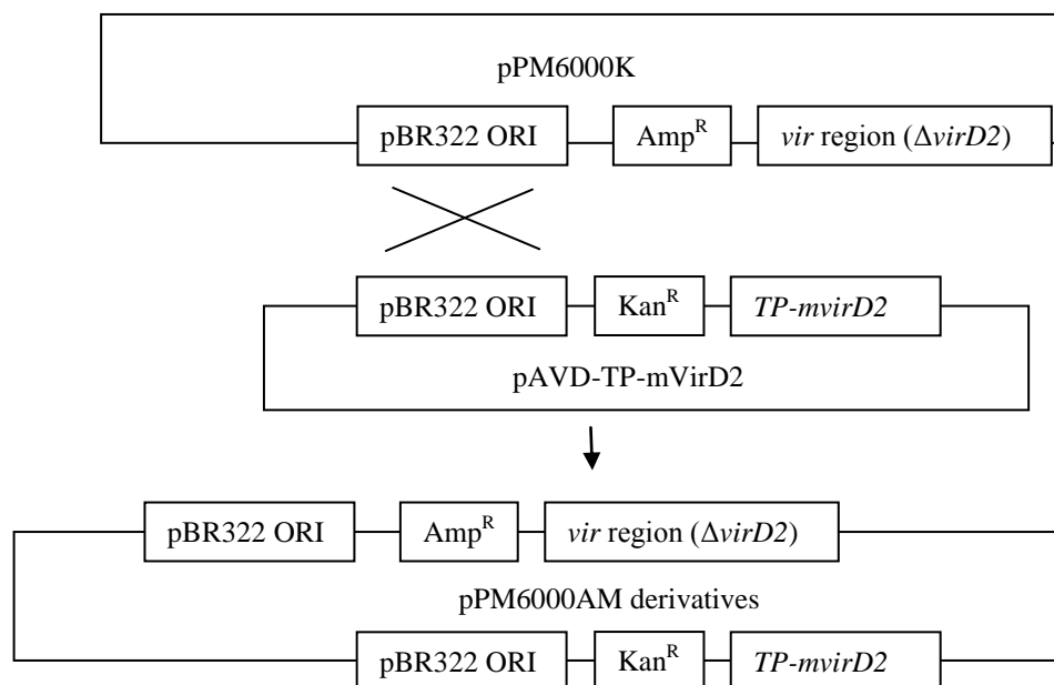
Figure 2.4.4.1.1. Construction of pPM6000AM derivatives.
