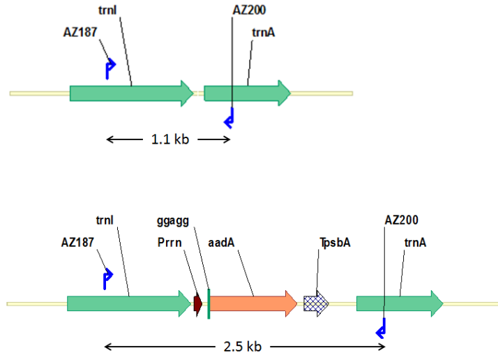
Figure 2.4.5. Top – The untransformed chloroplast genome. Bottom – the transformed chloroplast genome with the chloroplast expression cassette.
