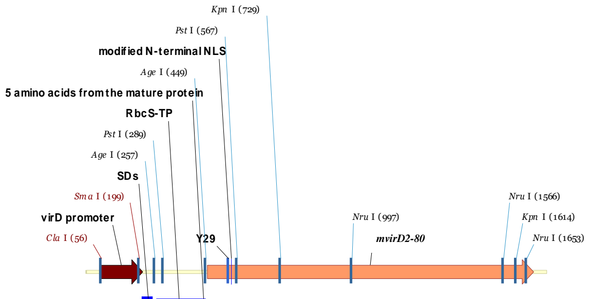
Figure 2.4.1e. Schematic representation of the RbcS-TP-mvirD2-80 gene in pVD80-RbcS-TP. SD: the Shine-Dalgarno sequence; some restriction sites are shown.
