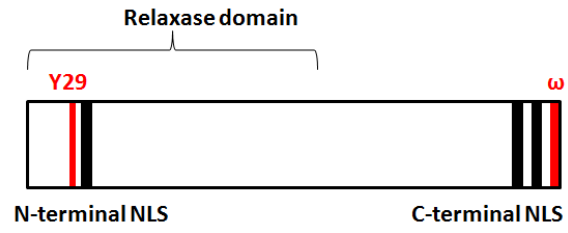
Figure 2.2a. Schematic representation of VirD2.
