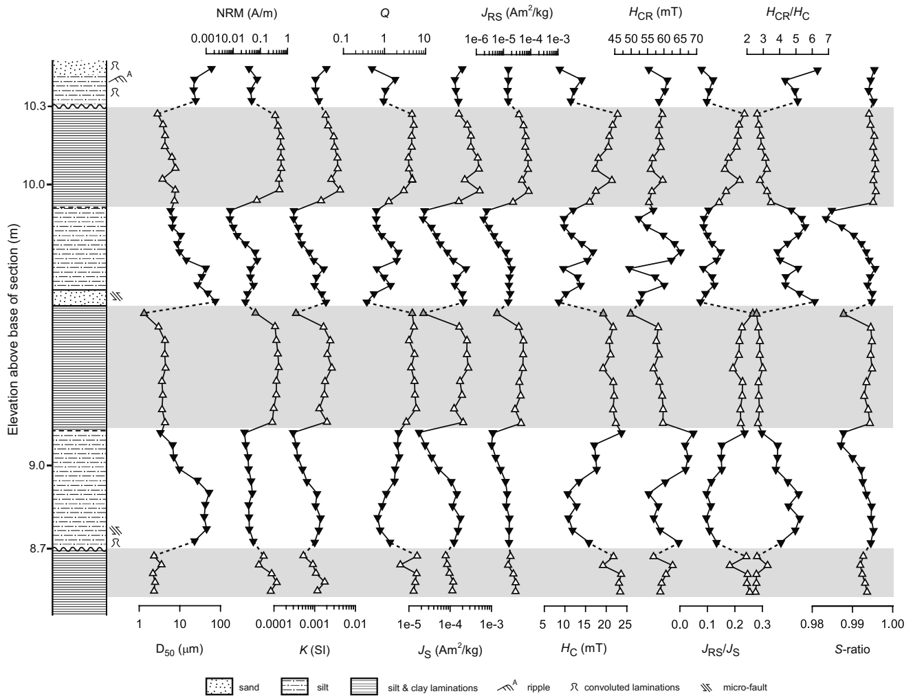
Figure 5. Results from samples collected through two units at Manila Creek. The stratigraphic column at the left shows major sedimentological units. Clay glaciolacustrine sediments are highlighted with gray banding and open triangles; closed upside-down triangles are flood sediments. Parameters displayed are median grain size ( D_{50} ), natural remanent magnetization (NRM), magnetic susceptibility ( K ), Koenigsberger ratio ( Q ), saturation magnetization ( J_S ), saturation remanence ( J_{RS} ), coercive force ( H_C ), coercivity of remanence ( H_{CR} ), and the S-ratio. One sample, highlighted in gray, is anomalous; see footnote 2 for details.
