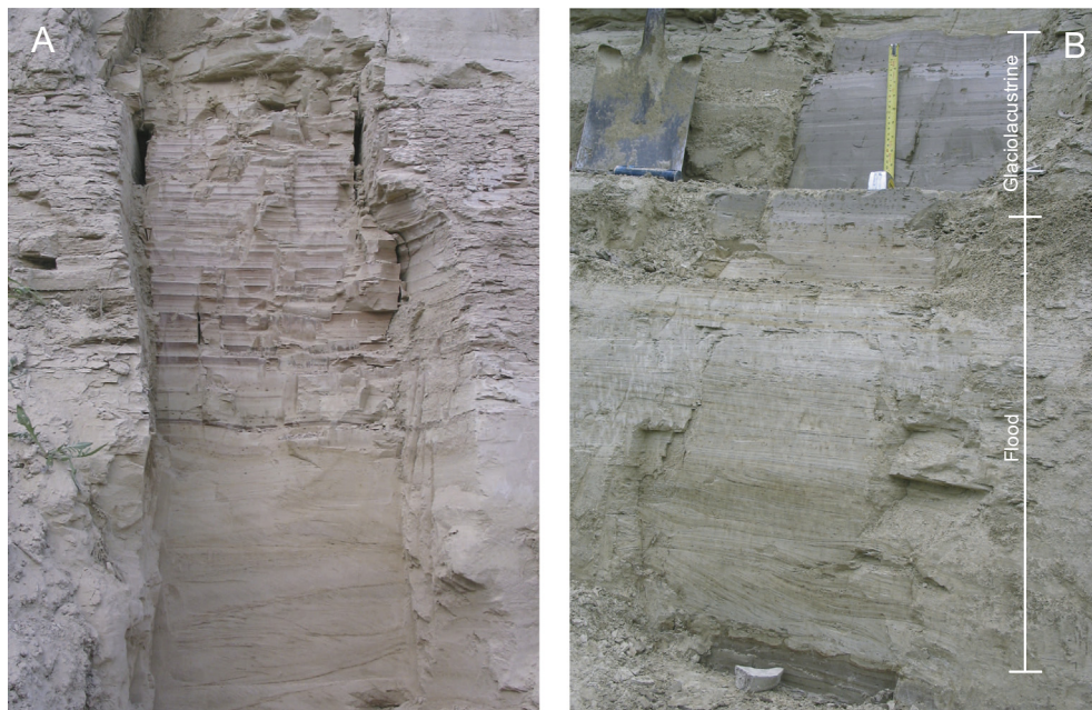
Figure 2. Photographs of units at each study site. (A) A single unit at Ninemile Creek that is about 3.3 m thick. The lower part of the unit consists of rippled and laminated fine sand and silt. This sediment grades upward into silt and clay varves. (B) One flood and one glaciolacustrine unit at Manila Creek. The lower flood sediment is characterized by a loaded lower contact and planar and inclined silt and clay laminations. The flood sediments grade up into glaciolacustrine, laminated clayey silt. The tape is about 30 cm long.
