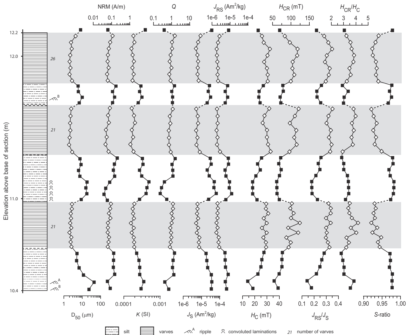
Figure 4. Magnetic results from samples collected through three glaciolacustrine units at Ninemile Creek. The stratigraphic column at the left shows major sedimentological units. Diamond symbols and gray banding are clay varved sediments; square symbols are silty sediments deposited by turbidity currents. Parameters displayed are median grain size ( D_{50} ), natural remanent magnetization (NRM), magnetic susceptibility ( K ), Koenigsberger ratio ( Q ), saturation magnetization ( J_S ), saturation remanence ( J_{RS} ), coercive force ( H_C ), coercivity of remanence ( H_{CR} ), and the S -ratio.
