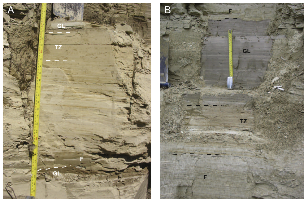
Figure 8. Flood (F) and glaciolacustrine (GL) sediments at Manila Creek. (A) The transition zone (TZ) between flood and glaciolacustrine sediments is characterized by massive, very fine silt to clay. (B) The transition zone (TZ) has a pinkish tinge similar to fine-grained, hematite-bearing, glacial Lake Missoula sediments at Ninemile Creek (see Fig. 2). (For interpretation of the references to color in this figure, the reader is referred to the web version of this article.)
