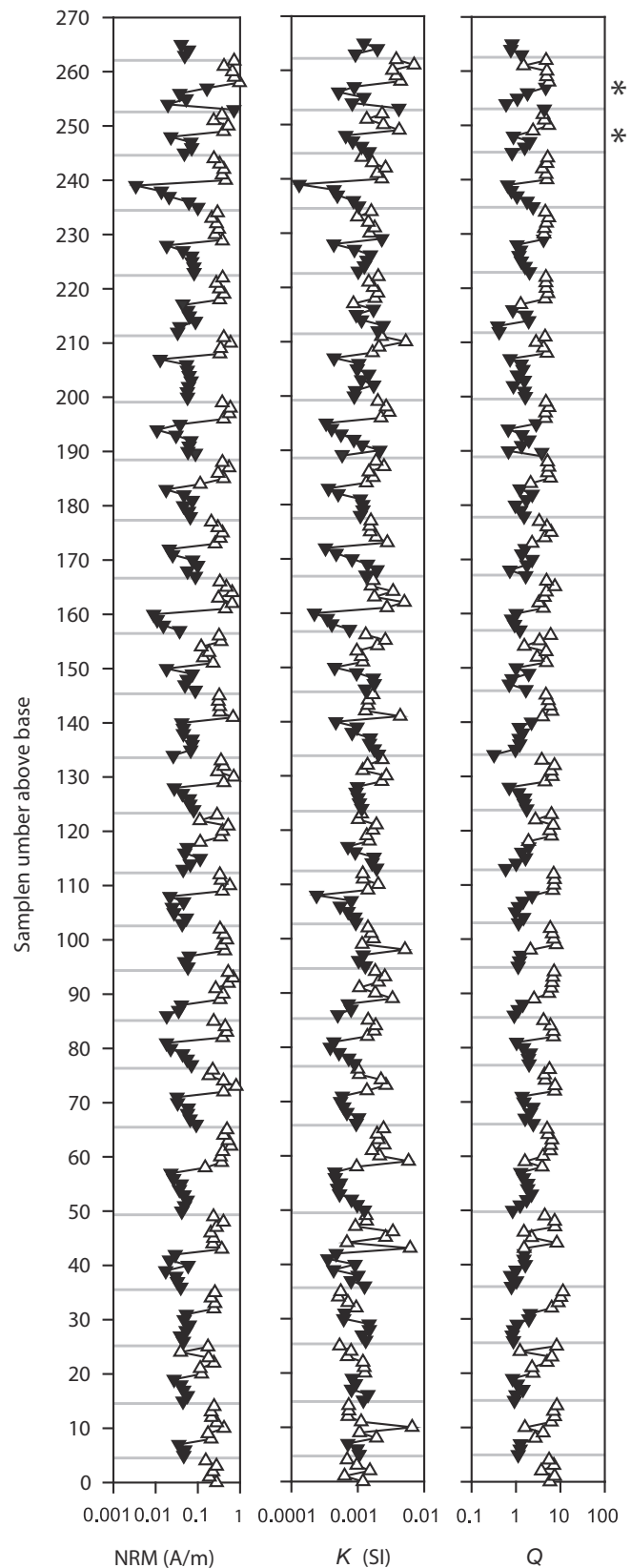
Figure 9. NRM, K , and Q for the lowest 25 units at Manila Creek. Glaciolacustrine samples are open triangles; flood samples are closed, upside-down triangles. Horizontal lines delineate the base of flood units. Note the gradual decrease in both NRM and K across erosional contacts at the base of the flood units and the sudden increase in NRM and K in the transition from flood units to glaciolacustrine units. The asterisks denote the two units in Fig. 6, although the samples represented here are from a different dataset that is not as detailed.
