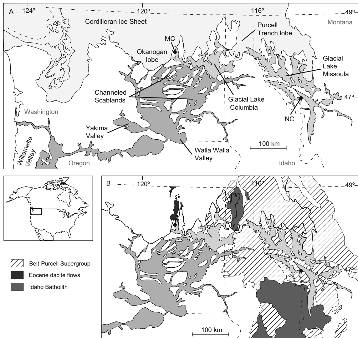
Figure 1. (A) Study area showing locations of sites mentioned in the text. MC: Manila Creek; NC: Ninemile Creek. Dark gray areas were swept by floodwaters from glacial Lake Missoula. Figure adapted from Waitt (1985), Atwater (1986), and Levish (1997). (B) Generalized, relevant geology of the study area (adapted from Stoffel, 1990; Vuke et al., 2007; Lewis et al., 2012).
