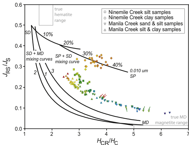
Figure 6. Hysteresis ratios for the two datasets shown on a Day plot. SD + MD and SP + SD mixing lines are from Dunlop (2002a). MD: multi-domain; SD: single domain; SP: superparamagnetic. The colors show a change in median grain size from 1.2 \mu\text{m} (red) to 78 \mu\text{m} (dark blue). The arrows indicate the top three samples in the two Manila Creek flood units (red = lower unit; green = upper unit). (For interpretation of the references to color in this figure, the reader is referred to the web version of this article.)
