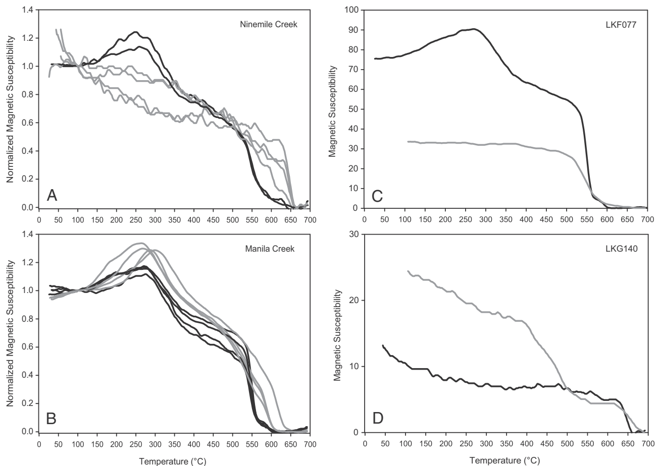
Figure 3. (A) and (B) Thermomagnetic curves from Ninemile Creek and Manila Creek, respectively. Curves of coarser-grained samples (turbidity currents at Ninemile Creek and flood units at Manila Creek) are black; curves of finer grained samples (glaciolacustrine units) are gray. To account for instrument drift, a small correction was applied to set the magnetic susceptibility to zero at high temperatures. We normalized susceptibility values to the susceptibility at 52°C, which is the highest starting temperature of any sample. (C) and (D) Examples of heating and cooling thermomagnetic curves from Manila Creek and Ninemile Creek, respectively. Black lines are heating curves; gray lines are cooling curves. To account for instrument drift, a small correction was applied to set the magnetic susceptibility to zero at high temperatures.
