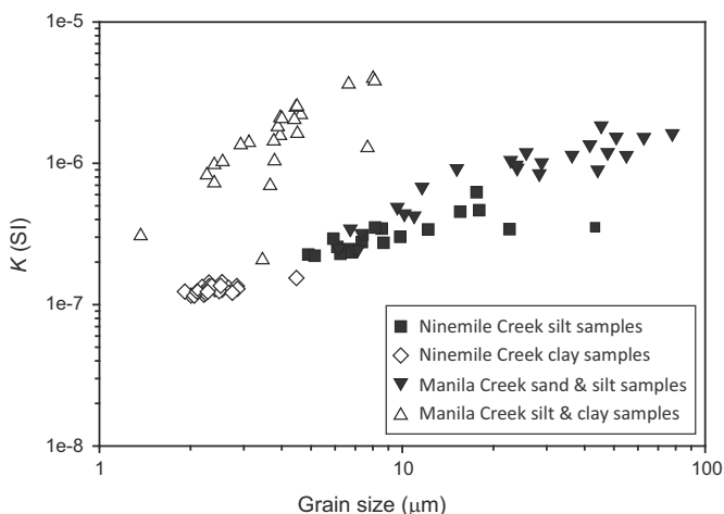
Figure 7. Plot of grain size vs. volumetric magnetic susceptibility ( K ). The linear trends indicate that the concentration of magnetite is directly proportional to grain size for each sediment type.
