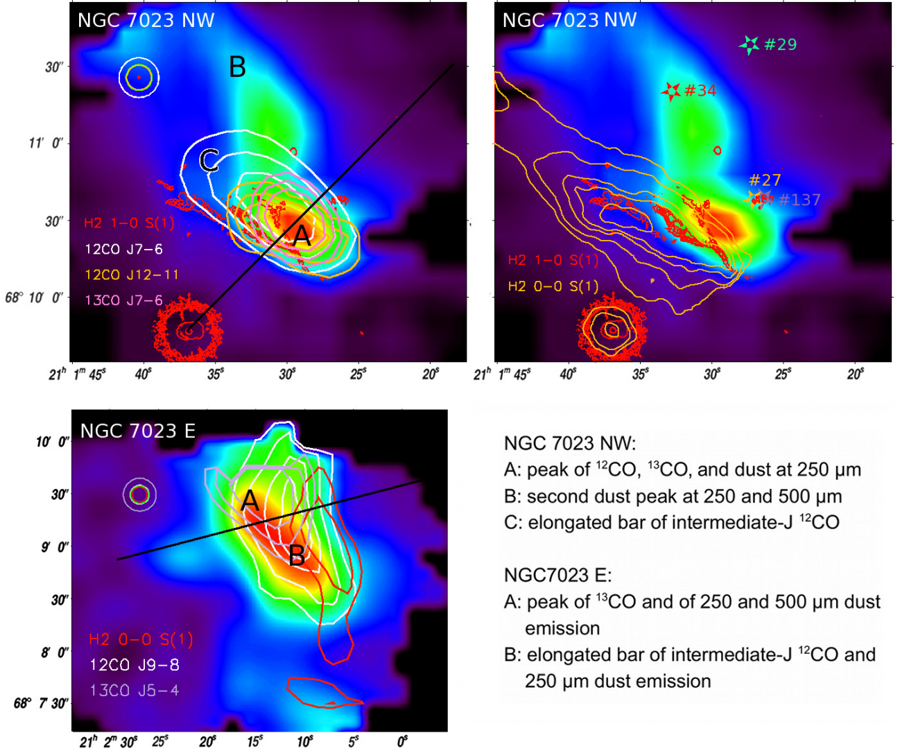
Fig. 6. Top left: FTS map at 250 μm of the PDR NGC 7023 NW with contours of 12 CO J = 7-6 (white), (maximum at 1.5 \times 10^{-5} erg cm -2 s -1 sr -1 with contour lines at 0.4, 0.6, 0.8 times the maximum), 12 CO J = 12-11 (orange) (maximum at 4.0 \times 10^{-5} erg cm -2 s -1 sr -1 with contour lines at 0.2, 0.4, 0.6 times the maximum), and 13 CO J = 7-6 (pink) (maximum at 3.2 \times 10^{-6} erg cm -2 s -1 sr -1 with contour lines at 0.4, 0.6, 0.8 times the maximum) and H 2 1-0 S(1) (red) from Lemaire et al. (1996) (maximum at 3.7 \times 10^{-4} erg cm -2 s -1 sr -1 with contours at 0.27, 0.41, 0.55, 0.69 times the maximum). Top right: FTS map at 250 μm of the PDR NGC 7023 NW with contours of H 2 0-0 S(1) (orange) from Spitzer observations (maximum at 1.9 \times 10^{-4} erg cm -2 s -1 sr -1 with contour lines at 0.26, 0.36, 0.52, 0.62, 0.83 times the maximum) and H 2 1-0 S(1) (red) (maximum at 3.7 \times 10^{-4} erg cm -2 s -1 sr -1 with contours at 0.27, 0.41, 0.55, 0.69 times the maximum). Bottom: FTS map of the PDR NGC 7023 E, 250 μm map with contours of 12 CO J = 9-8 (white) (maximum at 3.2 \times 10^{-6} erg cm -2 s -1 sr -1 with contour lines at 0.4, 0.6, 0.8 times the maximum), 13 CO J = 5-4 (violet) (maximum at 5.6 \times 10^{-7} erg cm -2 s -1 sr -1 with contour lines at 0.7, 0.8, 0.9 times the maximum) and H 2 0-0 S(1) (red) from Spitzer observations (maximum at 1.3 \times 10^{-4} erg cm -2 s -1 sr -1 with contour lines at 0.45, 0.66 times the maximum). Note that the FTS map at long wavelengths (SLW) is slightly smaller than the shown map, so that the 13 CO J = 5-4 contour lines are cut off in the north. The letters A, B, and C indicate positions of interest as explained. We include the detected YSOs by Kirk et al. (2009) as stars in the top right figure. The FWHM of the beam for the different CO and the beam size for H 2 lines are presented. Maps: 12.2'' (green). NGC 7023 NW: 11.6'' for 12 CO J = 12-11 (orange), 18.6'' for 12 CO J = 7-6 (white), 18.7'' for 13 CO J = 7-6 (white) and 1'' for H 2 1-0 S(1) (red). NGC 7023 E: 13.0'' for 12 CO J = 9-8 (white), 22.7'' for 13 CO J = 5-4 (violet) and 11'' for H 2 0-0 S(1) (red).
