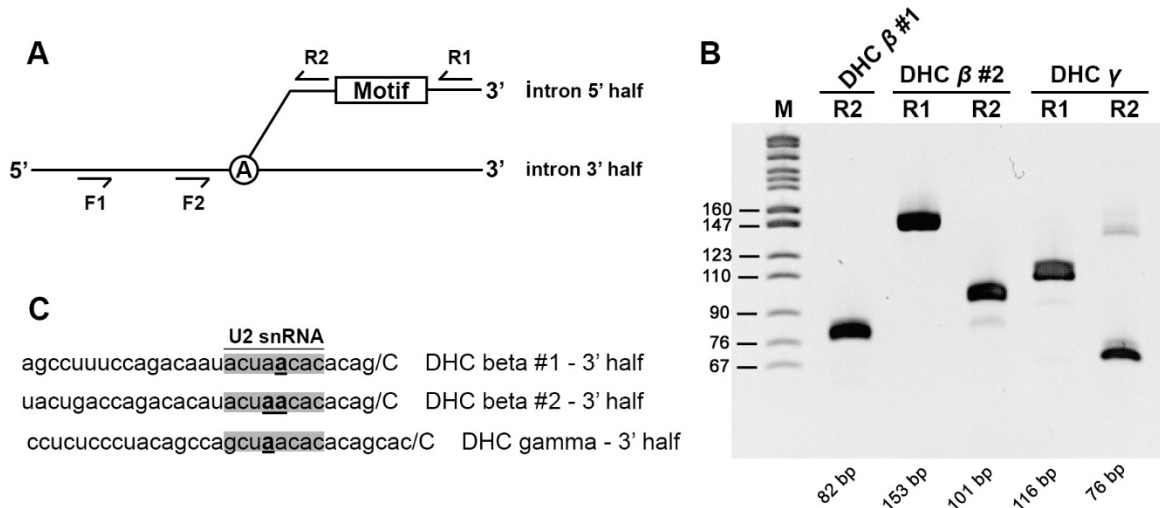
Figure 3.4. Detection of motif cleavage and BP nucleotides of G. lamblia trans -introns. (A) Experimental approach showing binding locations for forward (F1 and F2) and reverse (R1 and R2) primers used during RT-PCR. See Figure A.2.5A for more details. (B) RT-PCR products from nested PCR using F2 primers and reverse primers annealing downstream (R1) or upstream (R2) of the motif sequence. Names for trans introns and expected RT-PCR product sizes are shown above and below lanes, respectively. M = pBR322 Msp I size marker. Band sizes are indicated in base pairs (bp). (C) Branch point nucleotides determined by sequencing are indicated in bold text and underlined. Intron regions predicted to interact with U2 snRNA (Figure 3.10C) are highlighted in grey. See Figure A.2.5B for sequence traces confirming BP nucleotide positions.
