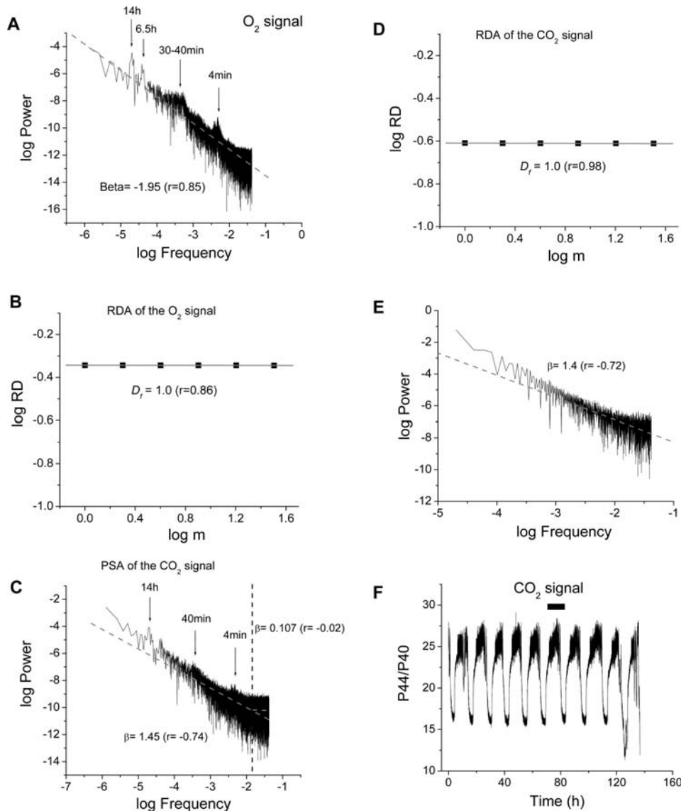
Figure 2. Relative Dispersional (RDA) and Power Spectral (PSA) Analysis of time series of O_2 and CO_2 signals obtained by MIMS from oscillating continuous cultures of S. cerevisiae . Both signals were processed for PSA (A, C, E) and RDA (B, D) under similar conditions as those described for heart mitochondria under Methods. The results obtained are in agreement with multiple dynamic, scale-free processes, exhibiting no predominant (characteristic) frequency. Interestingly, when the power spectrum, after Fast Fourier Transform (FFT) of the CO_2 time series, is performed on the “hairy” top of the oscillation (panel F; the bar in the inset indicates the portion of the time series analyzed), a similar \beta ( = 1.4 ; panel E) is obtained as in the case of the low frequency ( > 1 min period) domain of the spectrum ( \beta = 1.45 ; panel C). Clearly, the high frequency ( < 1 min period) domain corresponds to white noise ( \beta \sim 0.0 ) (panel C). Panel F shows the whole CO_2 time series analyzed. doi:10.1371/journal.pone.0003624.g002
