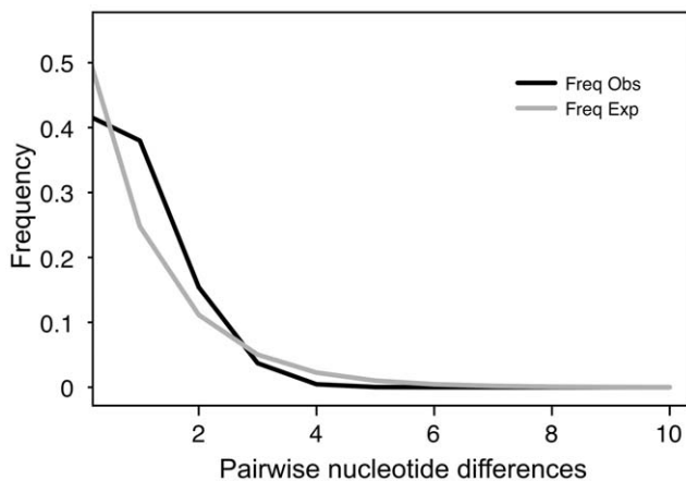
Figure 5. Mismatch distributions of pairwise nucleotide differences between mtDNA haplotypes revealed a unimodal pattern and no significant differences between the observed and expected frequencies (sum of squared deviation=0.000344, P=0.75 ). The black line is the observed frequency and gray line is the expected frequency. doi:10.1371/journal.pone.0040412.g005
